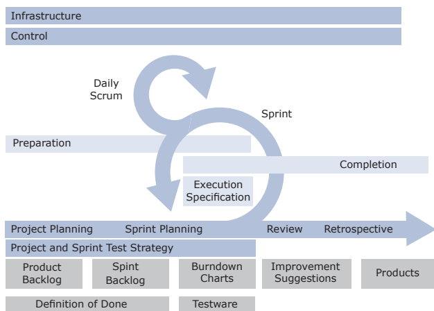
Abb.: TMap® lifecycle phases mapped on the Scrum model
