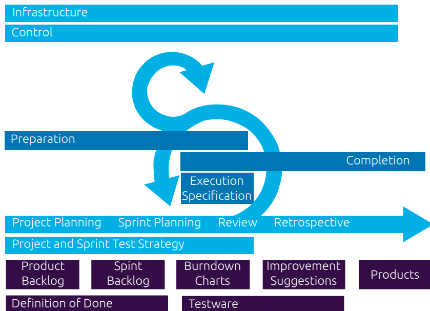
Abb.: TMap® lifecycle phases mapped on the Scrum model
